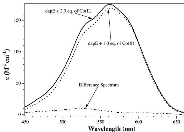
FIGURE 5: UV-vis spectra of Co(II)-substituted DapE at pH 7.5.
