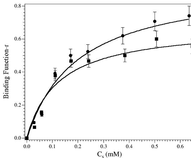
FIGURE 6: Plot of binding function r vs C_s (the concentration of free metal ions in solution) for the molar absorptivities at 562 nm (solid circles) and 532 nm (solid squares) for a 65 \mu M DapE sample in 50 mM HEPES buffer, pH 7.5.
