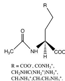
FIGURE 1: Acetylated amino acids.
