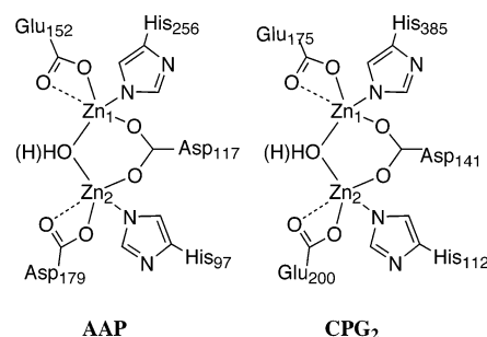
FIGURE 8: Active site drawings of AAP and CPG 2 .
